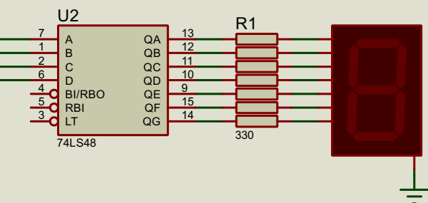
BCD-to-7-segment decoder/driver
