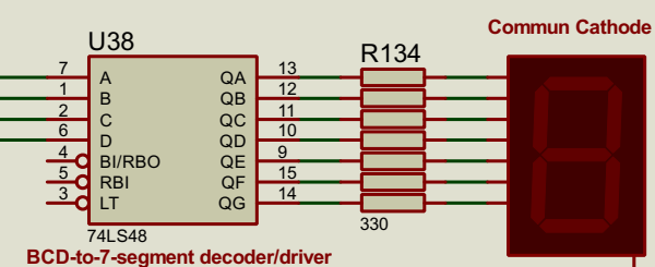
BCD-to-7-segment decoder/driver
