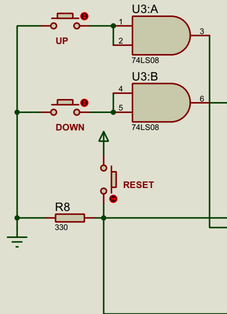
2-input AND gates with standard push-pull outputs
